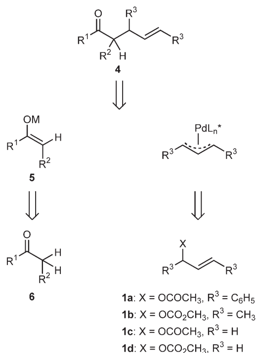
Scheme 2. Retrosynthesis of alkenyl ketones 4 based on ketones 6 and allylic substrates 1a–d via enolates 5 and allyl-palladium complexes. R 1 = alkyl, aryl, R 2 = alkyl.
