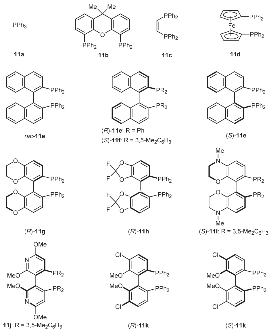
Scheme 4. Ligands used for stereoselective allylic alkylations of ketone enolates.
