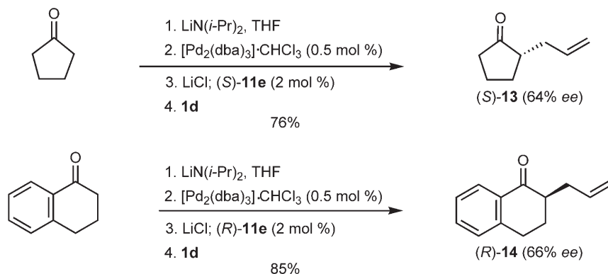
Scheme 6. Enantioselective allylation of cyclopentanone and \alpha -tetralone.
