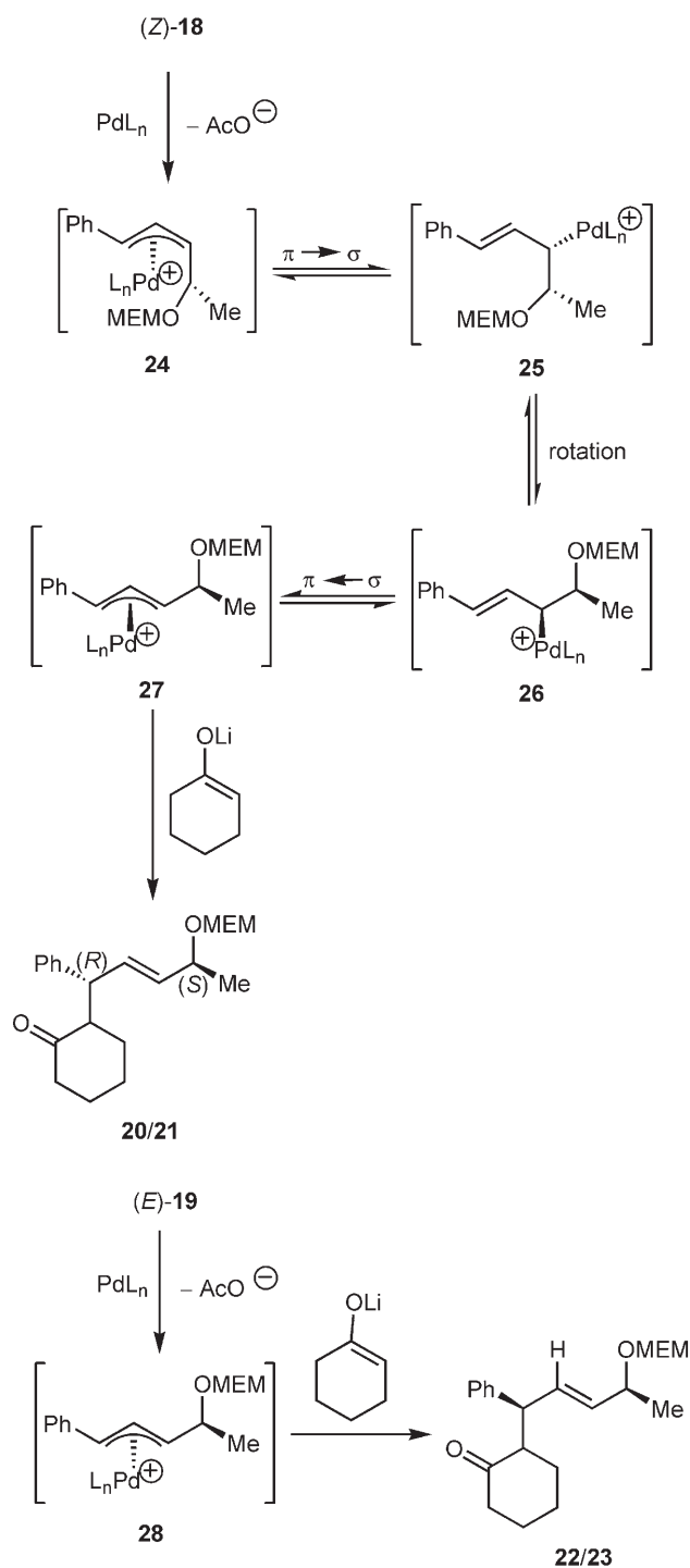
Scheme 9. Rationale for the stereochemical outcome in the reaction of allylic substrates ( Z )- 18 and ( E )- 19 with the lithium enolate of cyclohexanone.
