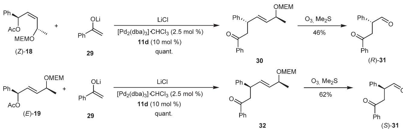
Scheme 10. Formation of diastereomeric products 30 and 32 from the palladium-catalyzed allylation of acetophenone with ( Z )- 18 and ( E )- 19 through the lithium enolate 29 .
