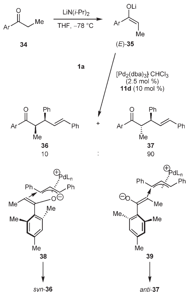
Scheme 12. Diastereoselective allylic alkylation of ethyl methyl ketone 34 and transition-state models.
