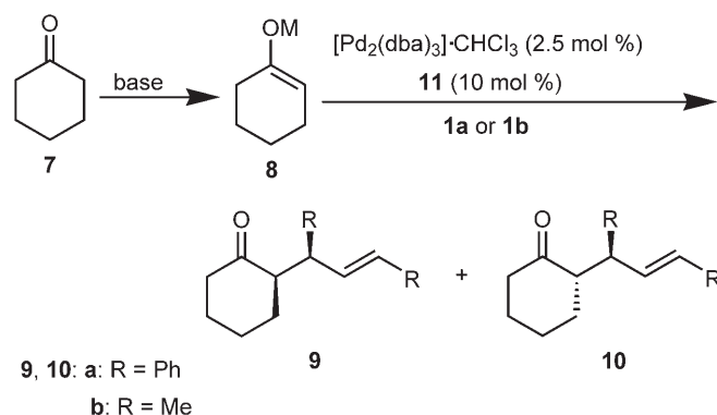
Scheme 3. Diastereoselective and enantioselective palladium-catalyzed allylic alkylation of cyclohexanone.
