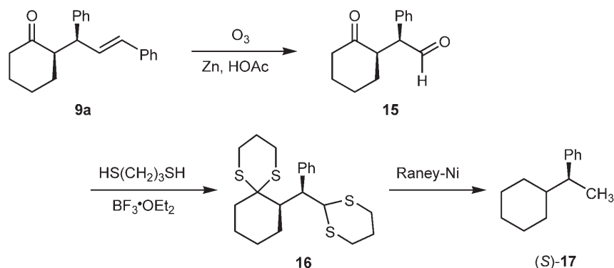
Scheme 7. Assignment of configuration to alkenyl ketone 9a by chemical correlation.
