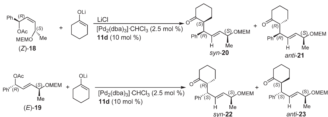
Scheme 8. Formation of diastereomeric products 20–23 from palladium-catalyzed reactions of cyclohexanone enolate with (Z) - 18 and (E) - 19 , respectively.
