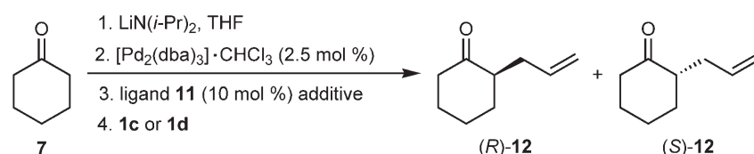
Scheme 5. Palladium-catalyzed enantioselective allylation of cyclohexanone.
