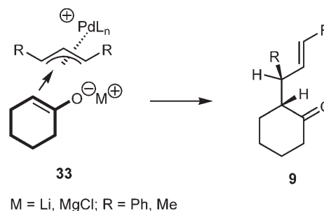
Scheme 11. Transition-state model for the diastereoselective allylic alkylation of cyclohexanone enolate 8 .
