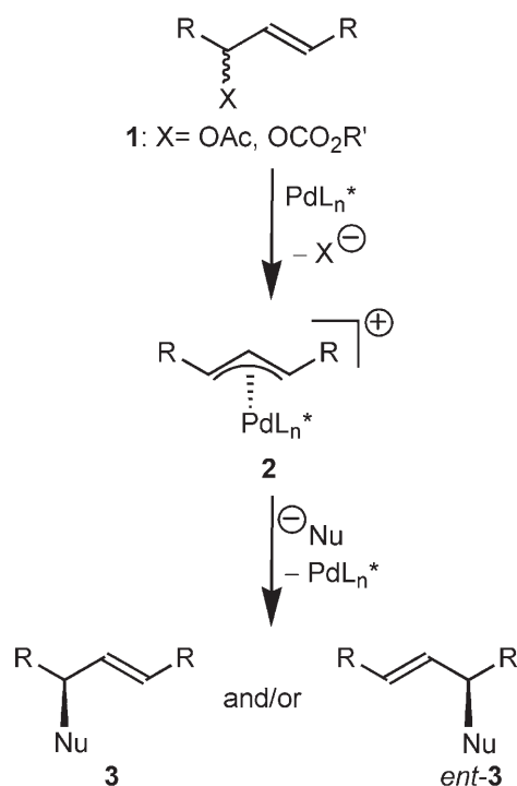
Scheme 1. “Standard” version of an enantioselective Tsuji-Trost allylic alkylation, Nu = CH(CO 2 R') 2 .
